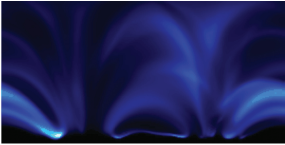
Figure 13: Image of coronal loops emulating TRACE observations at 195 nm. Courtesy of B. Gudiksen and A. Nordlund.
